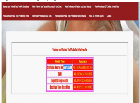
Fig2. Accuracy results
