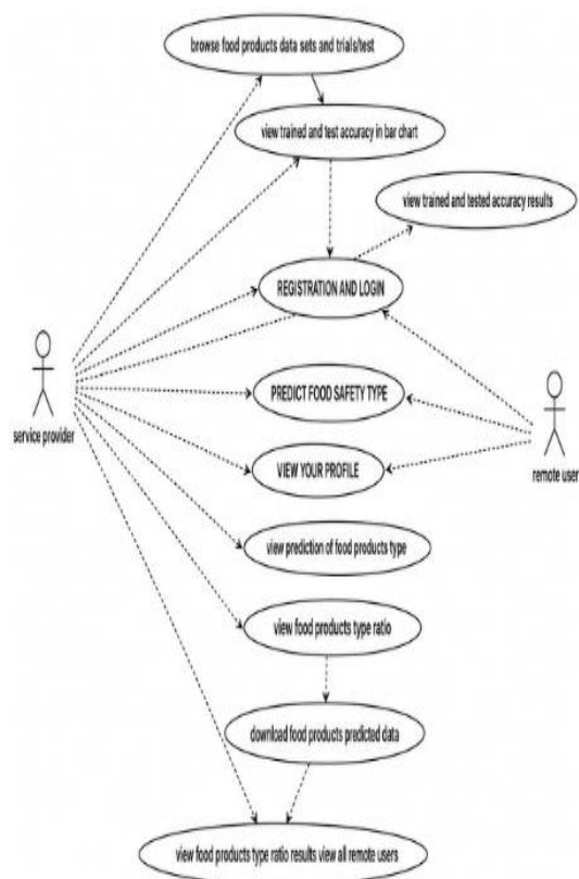
Fig.1. Food Safety Prediction Use Case Diagram
