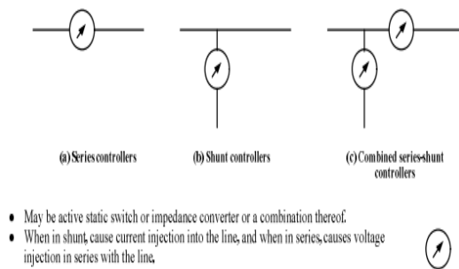
Figure1. Type of FACTS Controller
